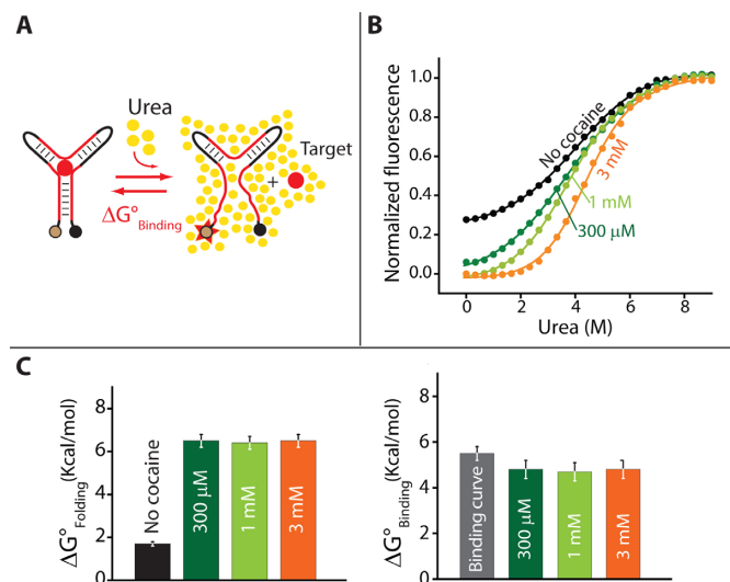
Figure 4. Determining the binding free energy of a DNA aptamer for its target. (A) Urea unfolding of the cocaine-binding aptamer. (B) Urea titration curves of the cocaine-binding aptamer in absence (black) and presence of different cocaine concentrations. (C) Comparison between folding and binding free energies of the cocaine-binding aptamer obtained using urea titration curves (at different concentrations of cocaine) and a classic binding curve (gray) (Supplementary Figures S12 and 13). The urea titration and binding curves were obtained in 50 mM sodium phosphate buffer, 500 mM NaCl, pH 7.0 at 25°C using 100 nM of aptamer.
